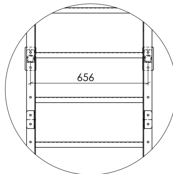
DETAIL AX SCALE 2 : 25
