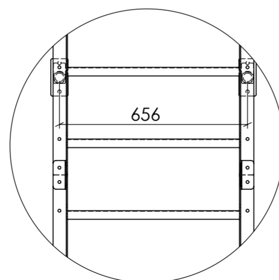
DETAIL AS SCALE 2 : 27
