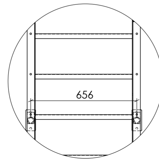
DETAIL BH SCALE 1 : 14
