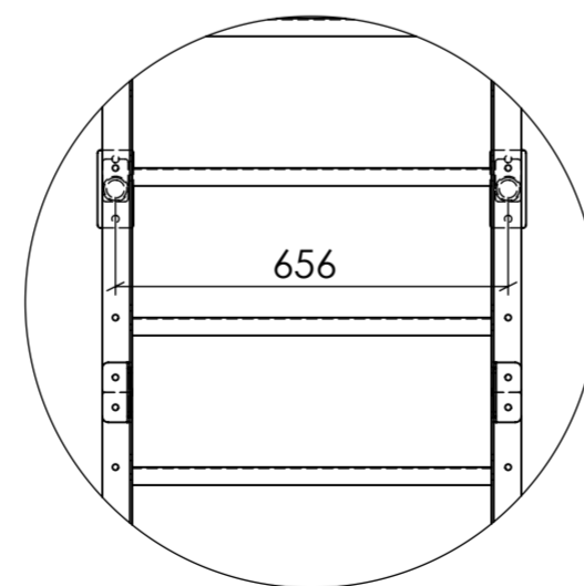
DETAIL BE SCALE 1 : 14
