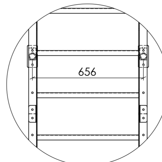
DETAIL BB SCALE 1 : 14
