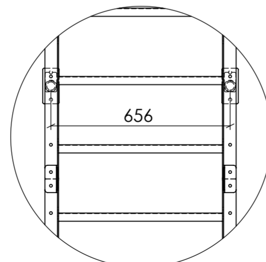
DETAIL BA SCALE 1 : 14
